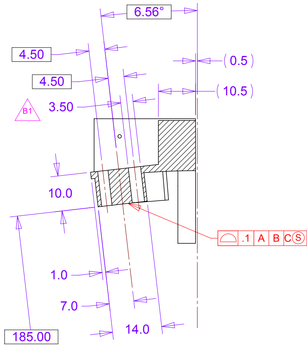
SECTION C-C
