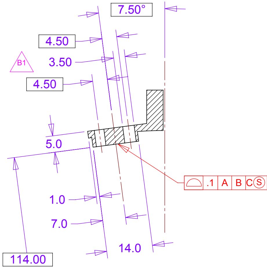
SECTION E-E
